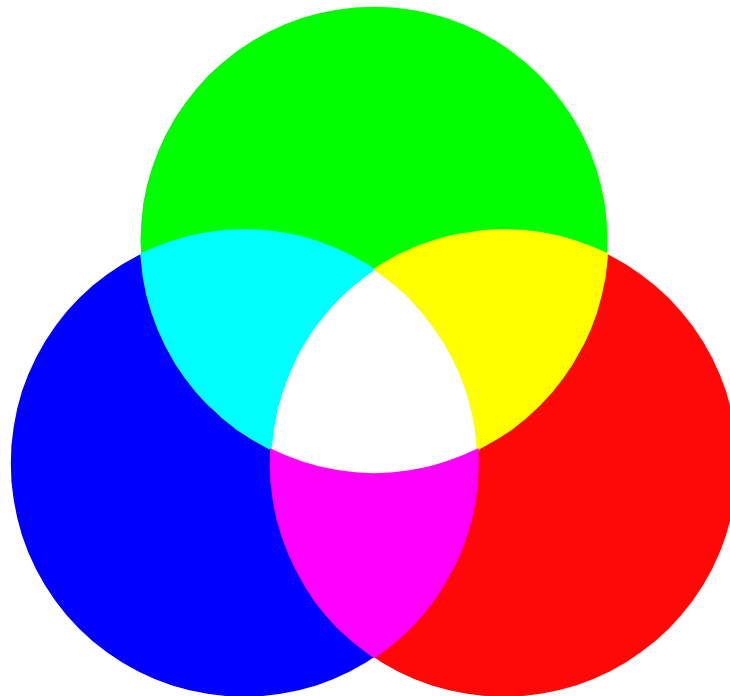
Figure 3. RGB model
